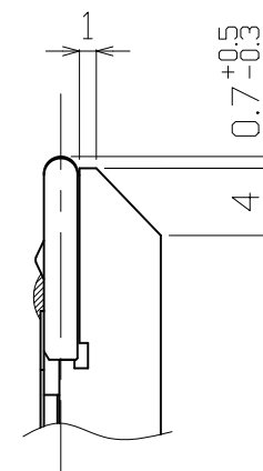
MAGNIFIED VIEW OF PART "A"
