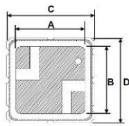
Monolithic Crystal Filter (MCF) Package
