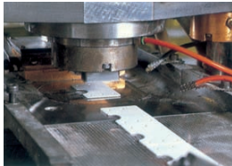
DRY PRESSING
