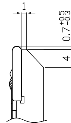
MAGNIFIED VIEW OF PART "A" (2/1)
