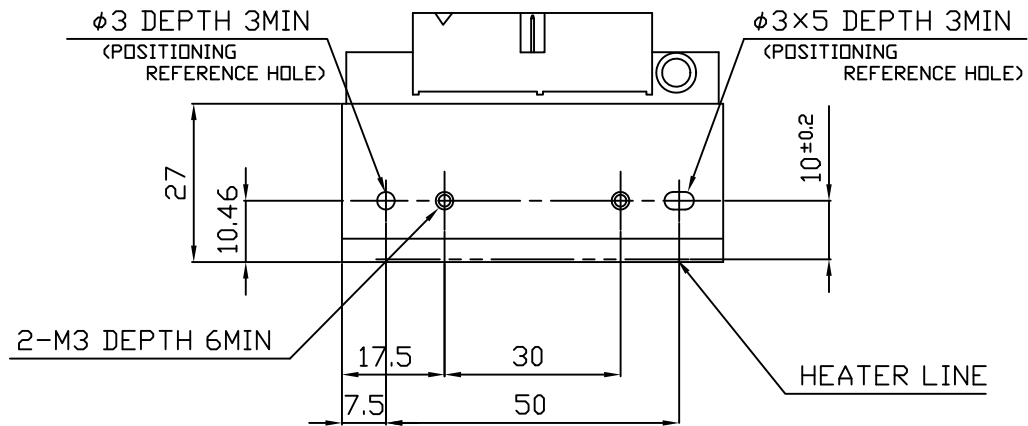
DETAIL "A"
