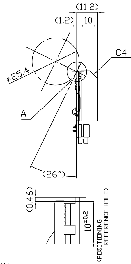
DETAIL "A"
