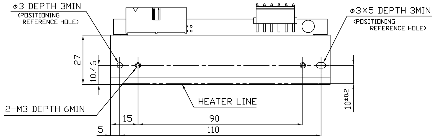
DETAIL "A"
