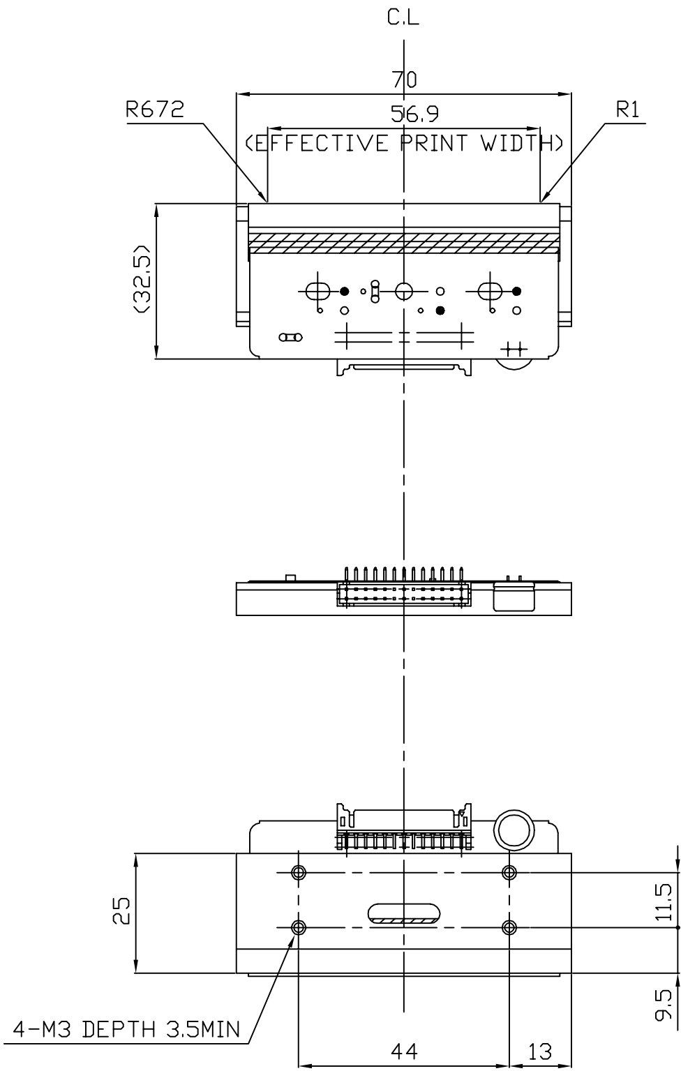
MAGNIFIED VIEW OF PART "A" (2/1)
