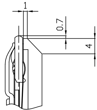
MAGNIFIED VIEW OF PART "A" (2/1)
